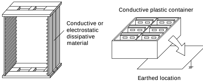
Fig. 5-23 Boad Storage Container
