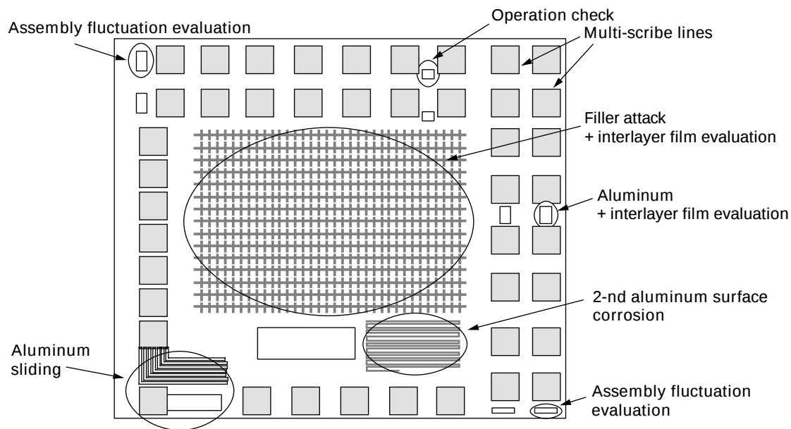
Fig. 4-5 Layout Image
