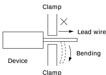
Fig. 5-26 Notes on Forming or Cutting External Leads
