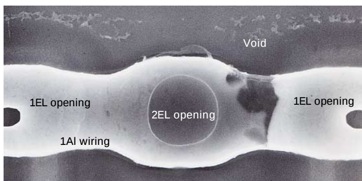
Photo 2-3 Disconnection Defect due to Stress Migration
