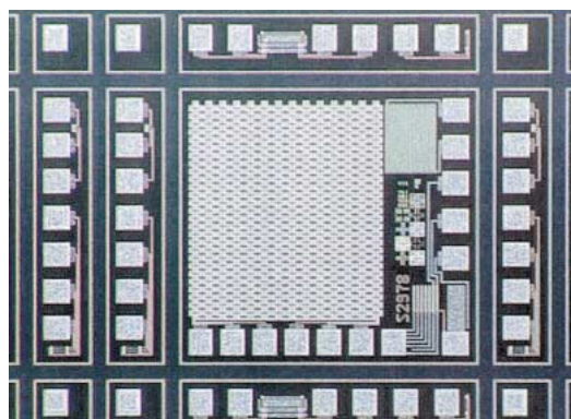
(b) TEG circuit block
