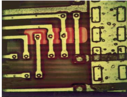
Photo 3-7 OBIC Analysis
