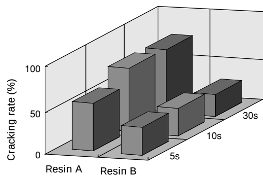
Fig. 5-11 Package Cracking Factor Confirmation Tests
