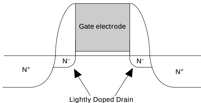
Fig. 2-3 LDD Structure
