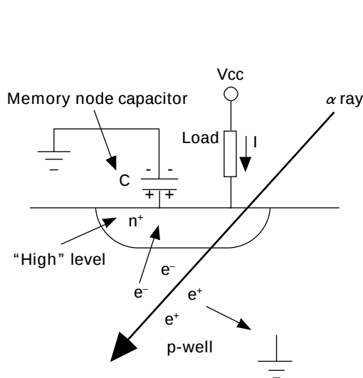
Fig. 2-9 Generation of Electron ( e^- ) and Hole ( e^+ ) Pairs by \alpha Rays
