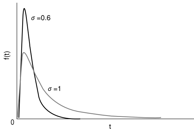
Fig. A-6 Logarithmic Normal Distribution
