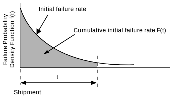
Fig. 4-8 Initial Failure Rate Curve and Cumulative Failure Rate up to Time t
