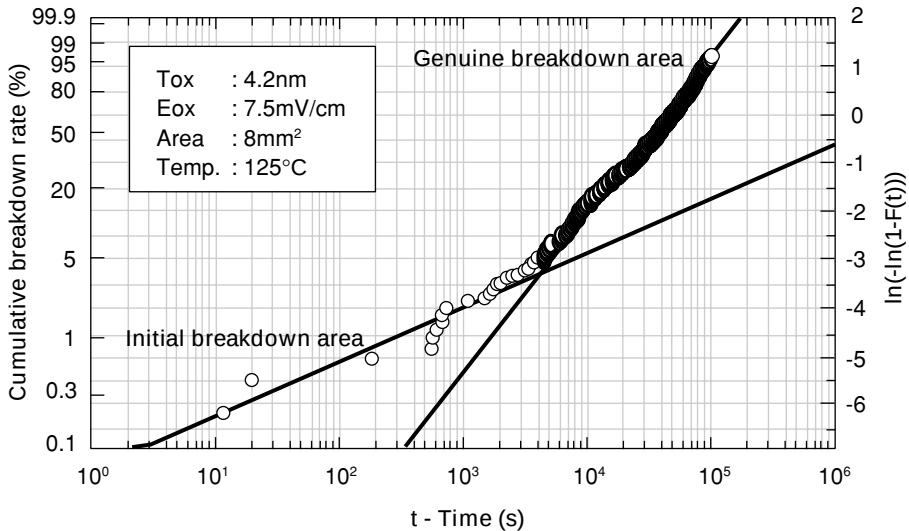
Fig. 2-4 TDDDB Characteristics at Constant Voltage
