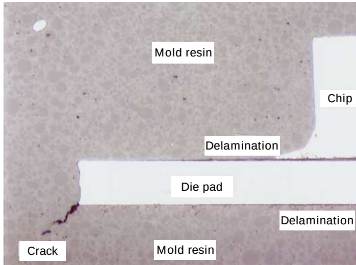
Photo 2-10 Package Cracking
