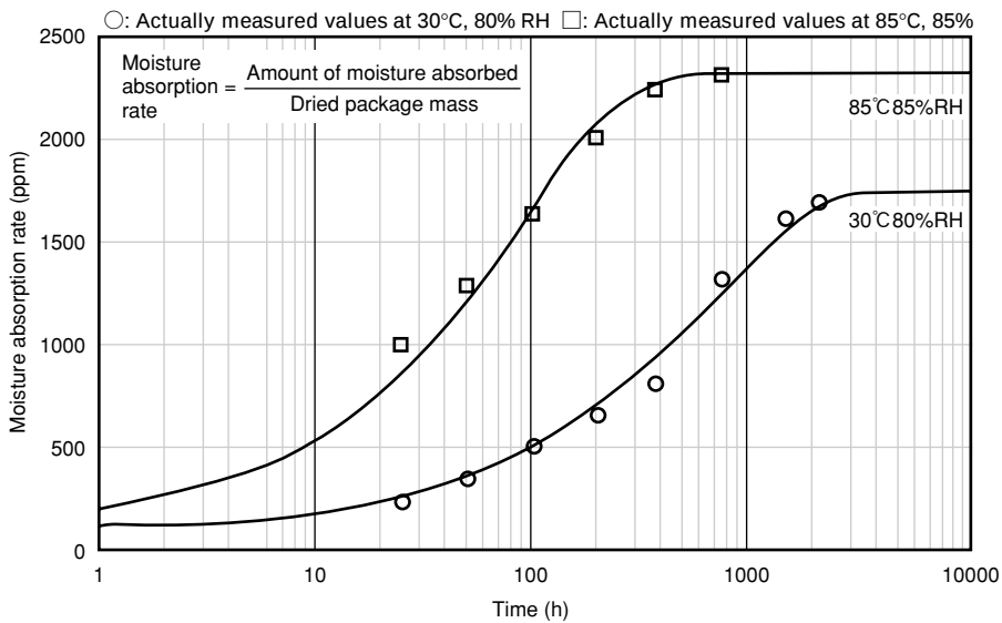
Fig. 5-3 Comparison of Theoretical Package Moisture Absorption Rate Curves with Actually Measured values for an 80-pin QFP
