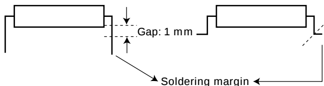
Fig. 5-36 Soldering Areas
