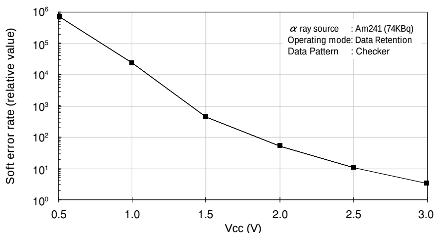
Fig. 2-11 Dependence of 8M SRAM Soft Error Rate on Supply Voltage
