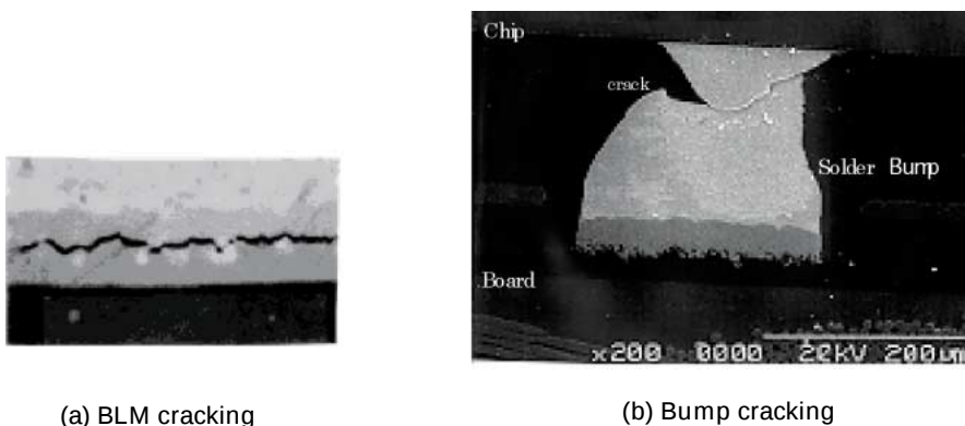
Photo 2-18 Failure Mechanisms in the Temperature Cycle Test
