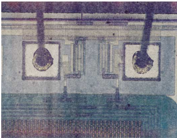
Photo 2-11 Aluminum Corrosion
