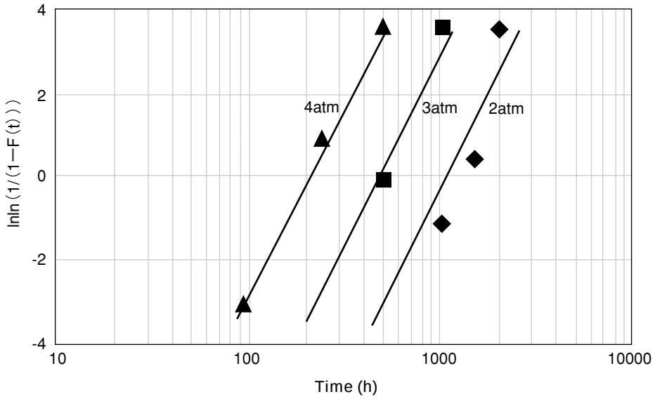
Fig. 4-20 Weibull Plot for Fuse Corrosion Failure
